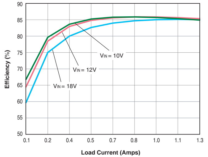
UWR-12/1250-D12A Efficiency vs. Line and Load
