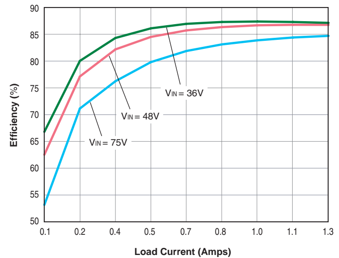
UWR-12/1250-D48A Efficiency vs. Line and Load
