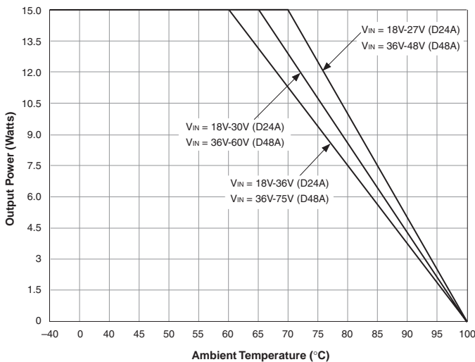
D24A and D48A Temperature Derating for 2.5V/12V/15V Output Models
