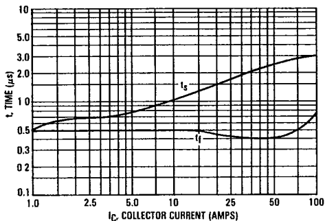
FIGURE 27 — TYPICAL TURN-OFF SWITCHING TIMES MJ10044
