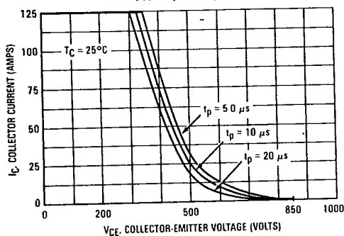
FIGURE 40 — OVERLOAD SAFE OPERATING AREA TYPE I (OLSOA) MJ10044
