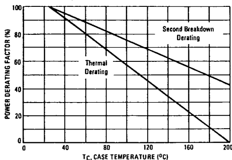
FIGURE 28 — POWER DERATING
