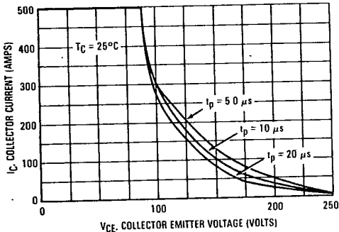
FIGURE 42 — OVERLOAD SAFE OPERATING AREA TYPE I (OLSOA) MJ10047
