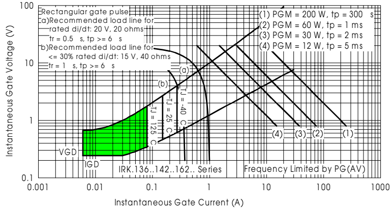
Fig. 34 - Gate Characteristics
