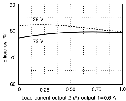
Efficiency (typ) @ T_A = +25^\circ\text{C}
