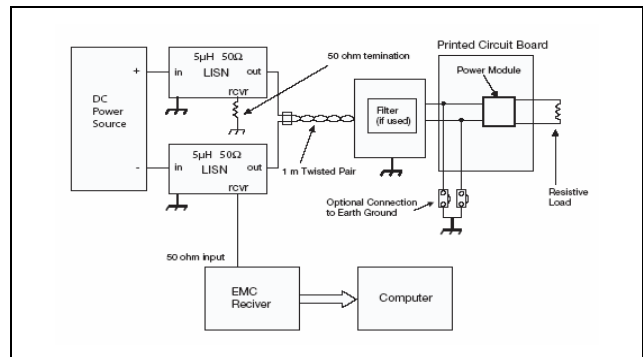
Test set-up
