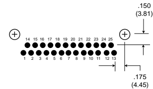
25 Contacts
