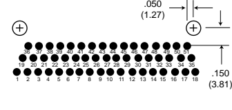
51 Contacts
