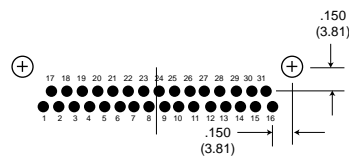
31 Contacts
