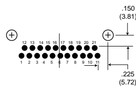
21 Contacts
