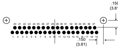
37 Contacts
