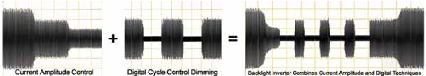
Figure 2 – LXM1614 Combines Current Amplitude and Digital Techniques
