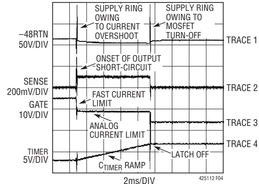
Figure 4. Output Short-Circuit Behavior (All Waveforms are Referenced to V_{EE} )
