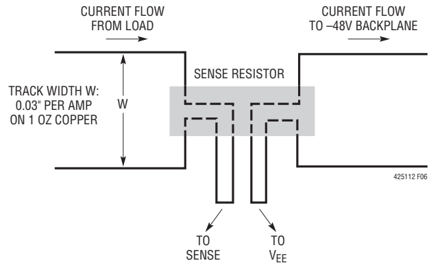
Figure 6. Making PCB Connections to the Sense Resistor
