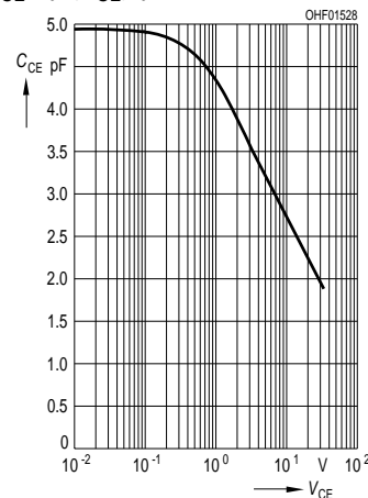
Capacitance
