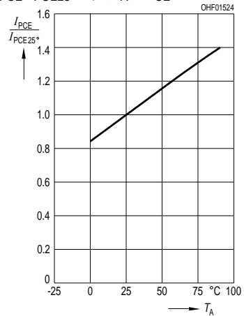
Photocurrent
