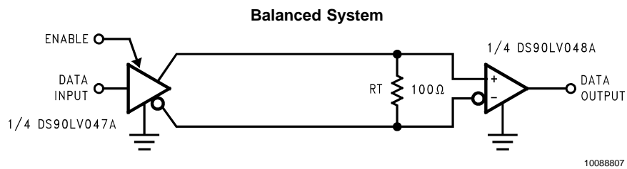
FIGURE 5. Point-to-Point Application
