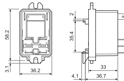
066.07 with relay
