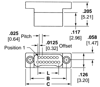
Plug
