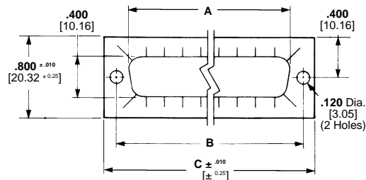
9, 15, 25 and 37 Positions
