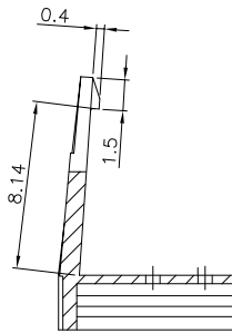
SECTION Z-Z
