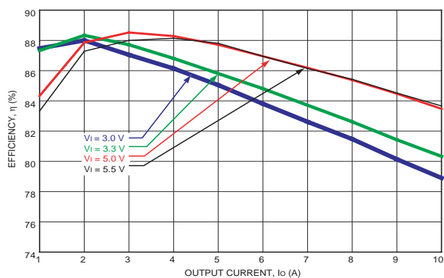
Figure 3. Converter Efficiency vs output current AXH010A0S0R9-SR(0.9V Output Voltage).
