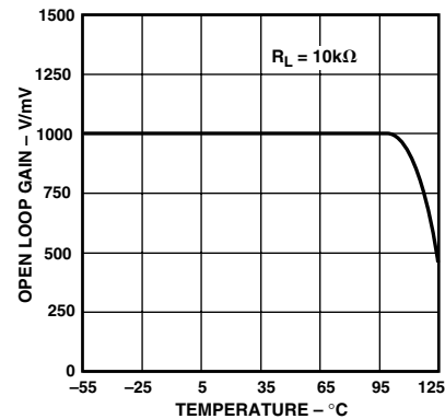
TPC 9. Open-Loop Gain vs. Temperature
