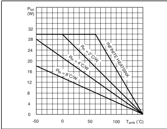
Figure 18. Maximum allowable power dissipation vs. ambient temperature
