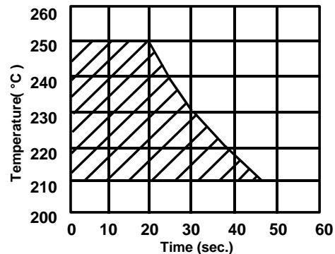
<Allowable Reflow Soldering Temp. and Time>
