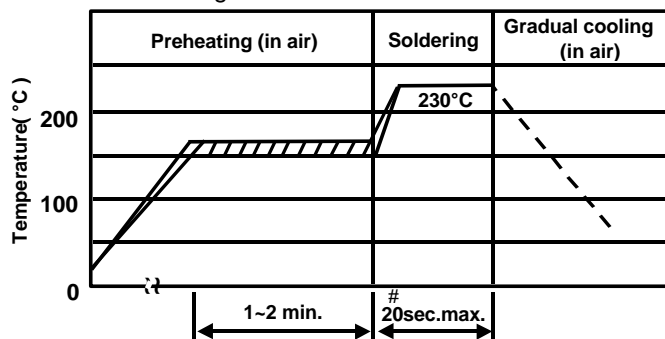
<Reflow Soldering Condition>
