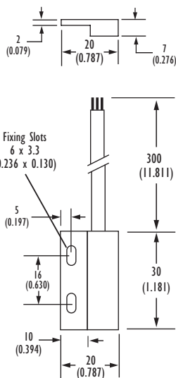
Drawings not to scale All dimensions in mm(inches) nominal
