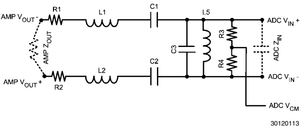
FIGURE 17. Sample Bandpass Filter
