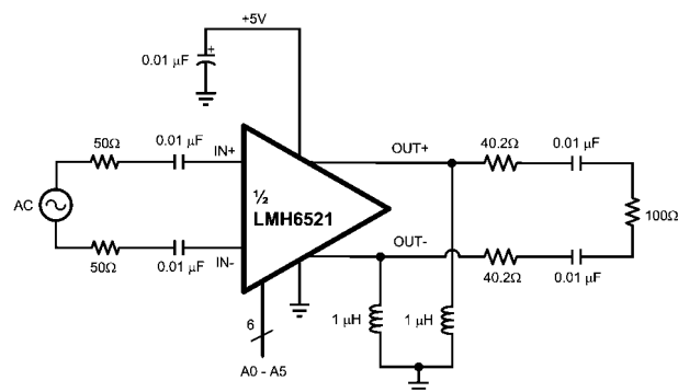
FIGURE 2. Basic Operating Connection
