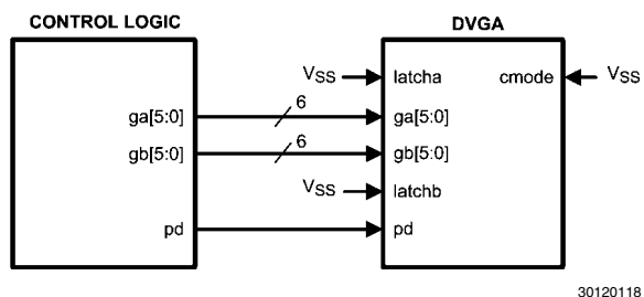
FIGURE 8. Parallel Mode Connection Not Using Latch Pins (Latch pins tied to logic low state)
