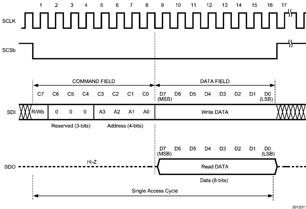
FIGURE 10. Serial Interface Protocol (SPI compatible)
