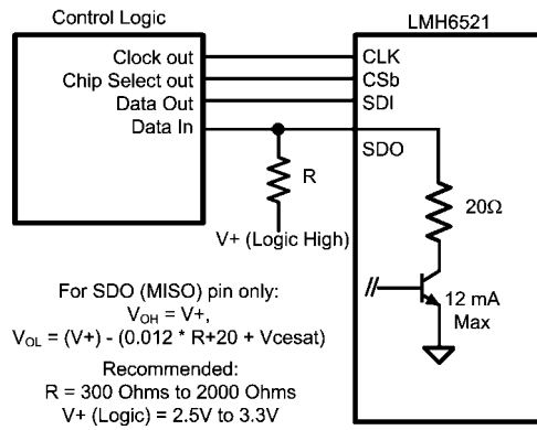
FIGURE 11. Serial Mode 4-wire Connection
