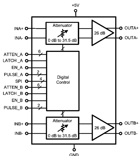
FIGURE 3. LMH6521 Block Diagram
