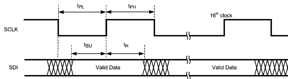
FIGURE 13. Write Timing Data Written to SDI Pin
