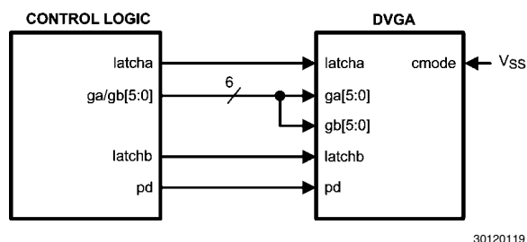
FIGURE 9. Parallel Mode Connection Using Latch Pins to Mux Digital Data
