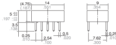
Self-clinching terminal
