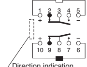
2-coil latching
