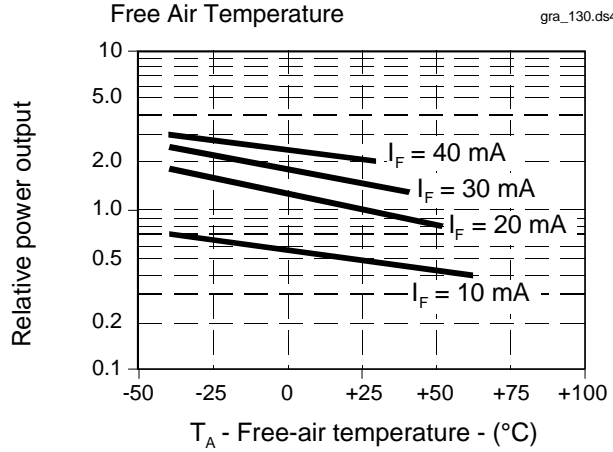
Fig. 7 Relative Power Output vs Free Air Temperature
