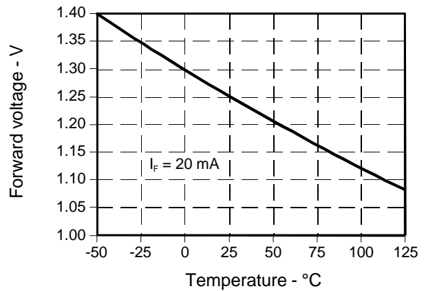
Fig. 4 Forward Voltage vs Temperature gra_200.ds4
