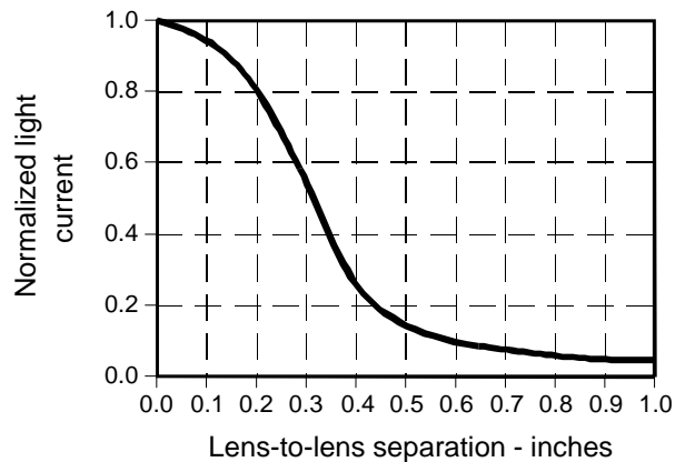
Fig. 6 Coupling Characteristics with SD1440 gra_006.ds4
