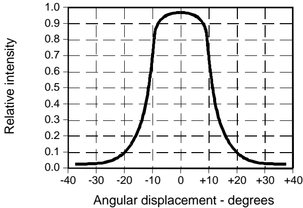
Fig. 1 Radiant Intensity vs Angular Displacement gra_001.ds4
