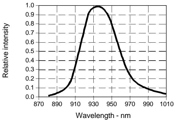
Fig. 5 Spectral Bandwidth gra_005.ds4
