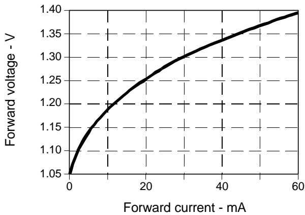
Fig. 3 Forward Voltage vs Forward Current gra_003.ds4
