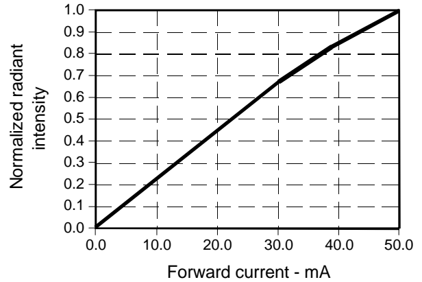
Fig. 2 Radiant Intensity vs Forward Current gra_002.ds4
