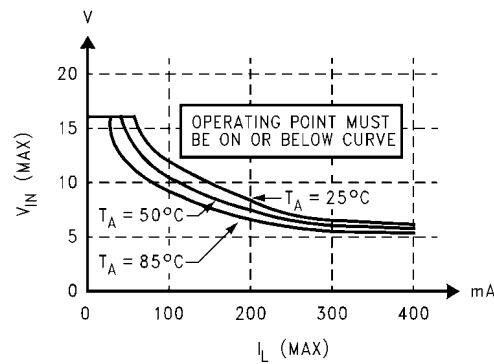
FIGURE 7. Safe Operation Boundary Curves for Figure 6
