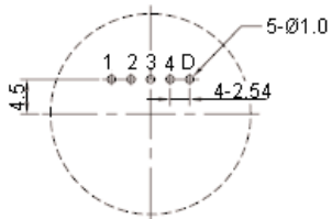
5 Pin Wafer PCB Layout
