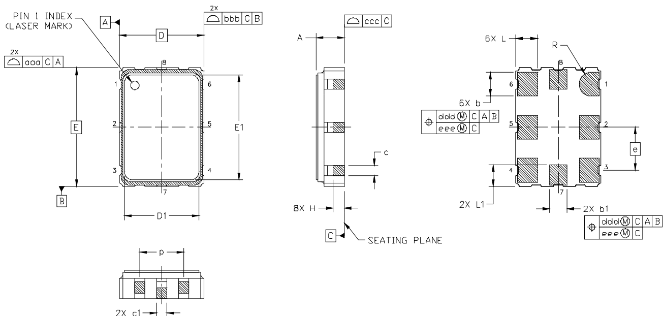
Figure 8. Si570/Si571 Outline Diagram
