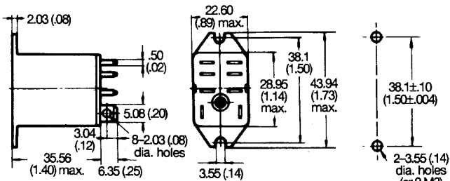
Mounting holes
