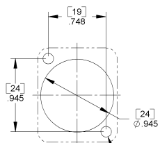
PANEL CUT-OUT FRONT OR REAR MOUNT
