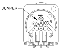
FEMALE CONNECTOR GROUND TO PIN # 1 OPTION "G1"
