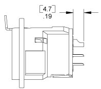
FEMALE SOLDER CUP OPTION "SC"
