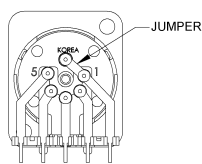
MALE CONNECTOR GROUND TO PIN # 1 OPTION "G1"
