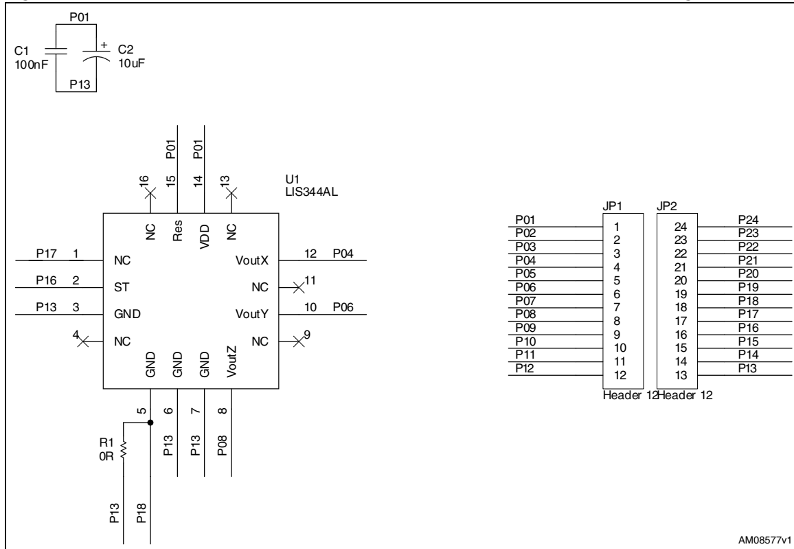
Figure 1. STEVAL-MKI017V1 demonstration board schematic and connection diagram
