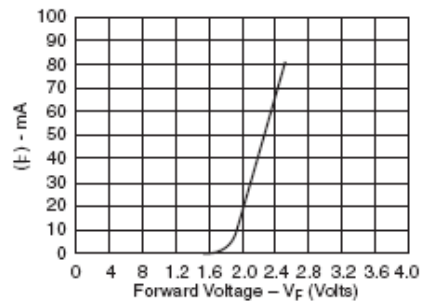
Fig. 4B. Forward Current vs. Forward Voltage
