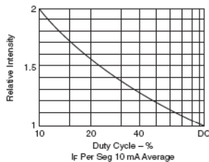
Fig. 4E. Relative Luminous Intensity vs. Duty Cycle
