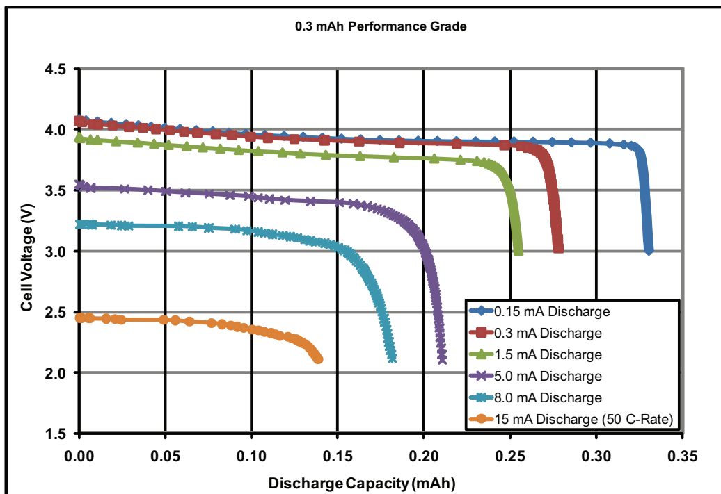
Figure 2: Typical Discharge Curves @25°C (300 µAh Performance Grade Cell)
