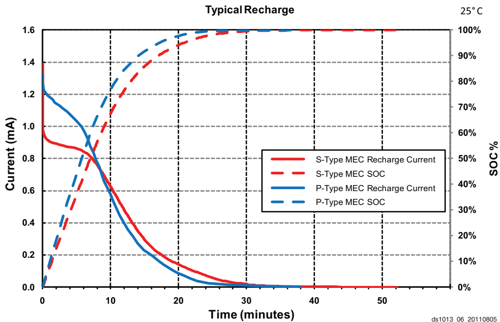
Figure 6: Typical Charge Curve @ 25°C — All Capacity Options
