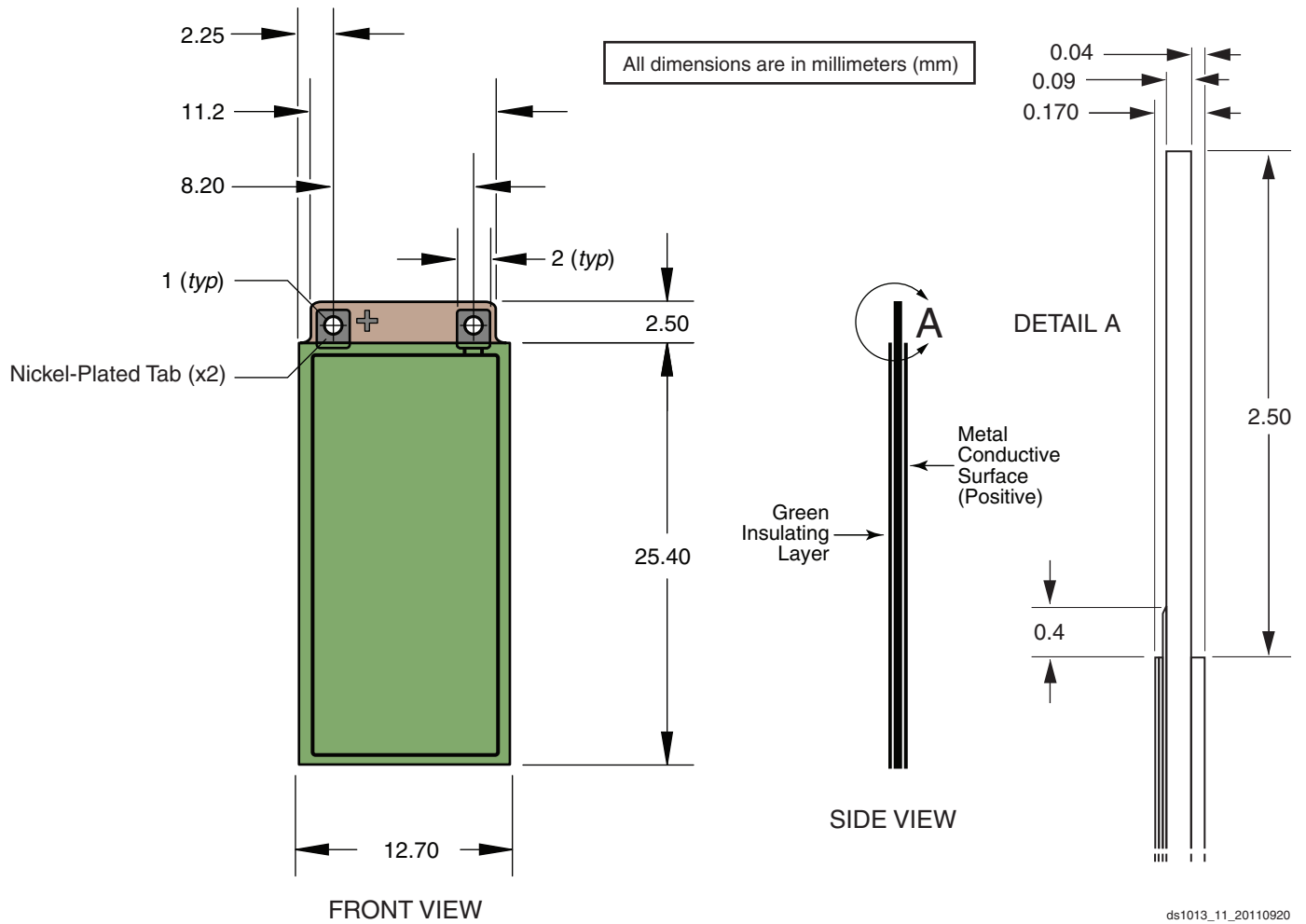
Figure 11: Front and Side Views
