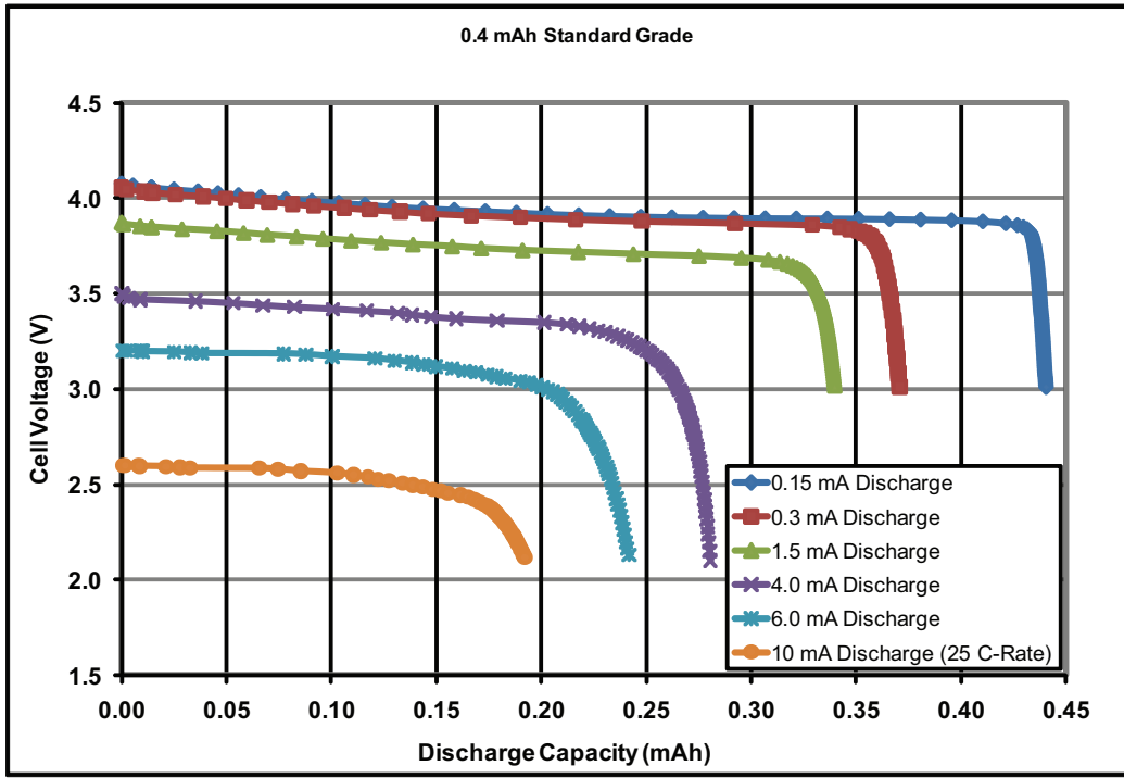
Figure 3: Typical Discharge Curves @25°C (400 µAh Standard Grade Cell)
