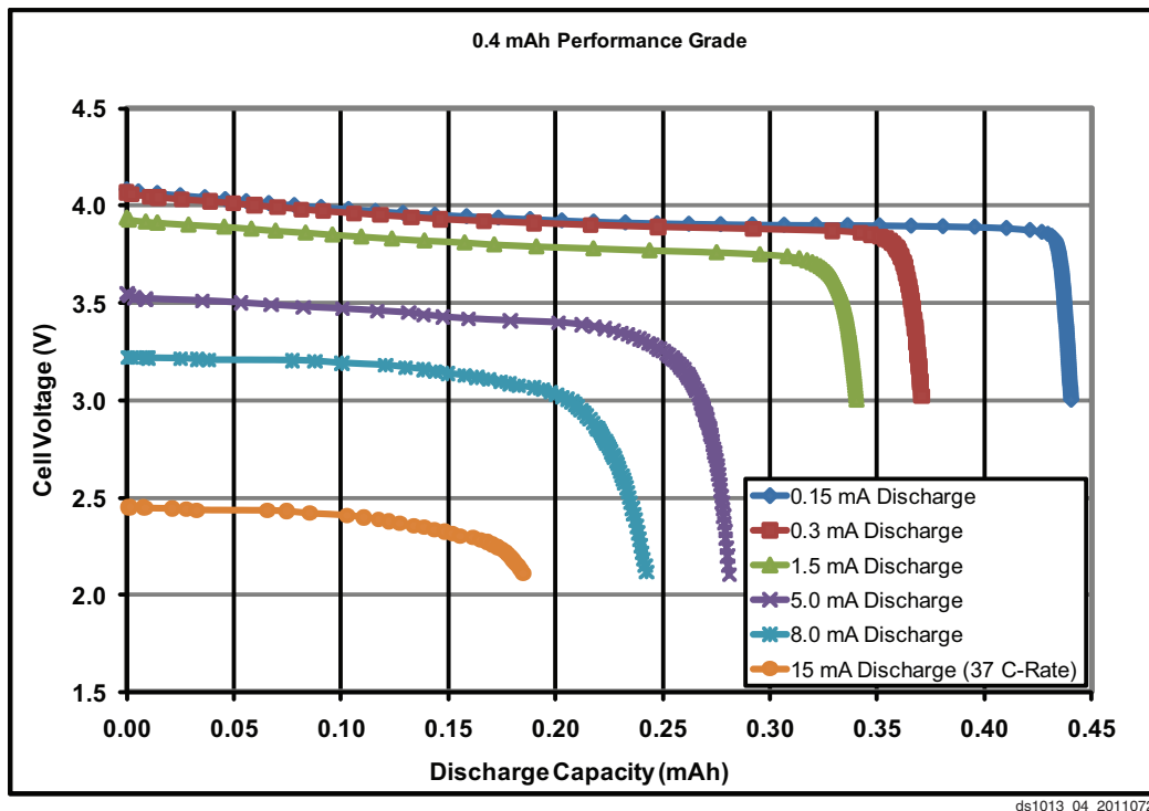
Figure 4: Typical Discharge Curves @25°C (400 µAh Performance Grade Cell)
