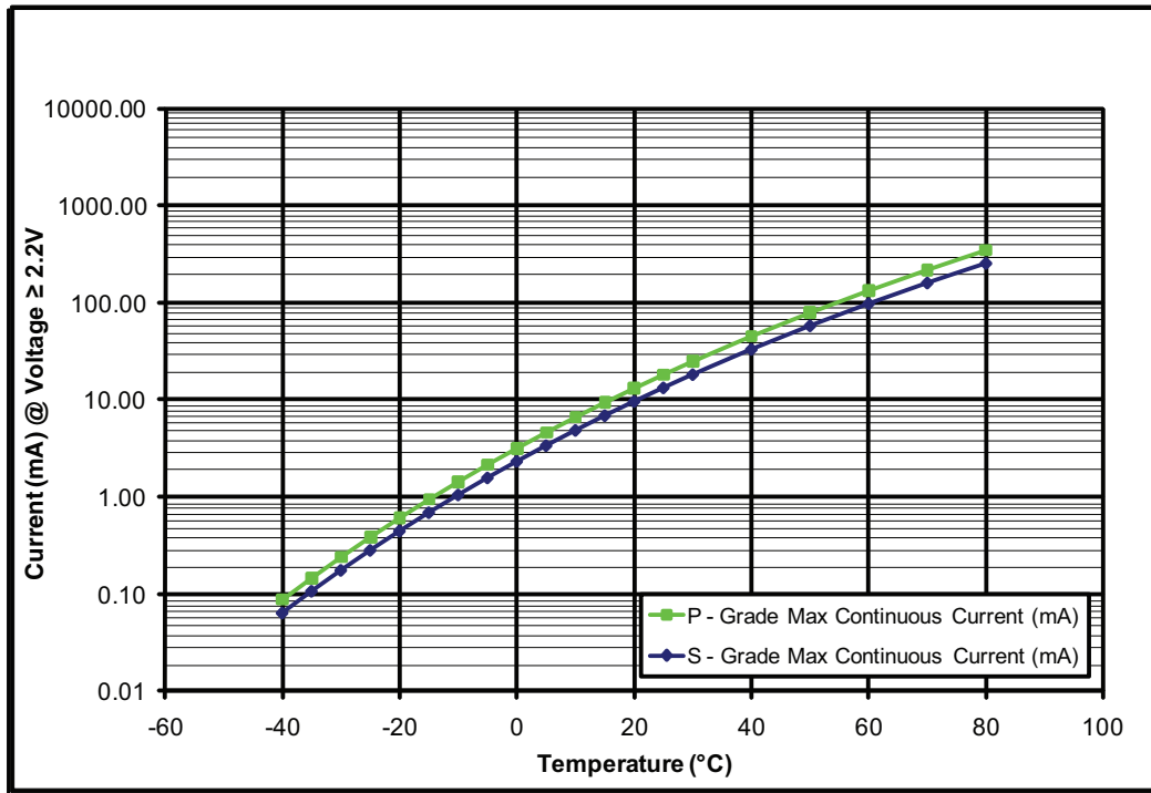
Figure 5: Typical Maximum Current vs. Temperature — All Capacity Options
