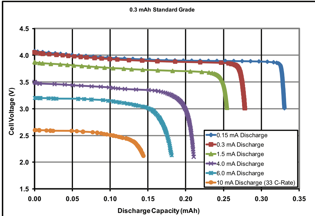
Figure 1: Typical Discharge Curves @25°C (300 µAh Standard Grade Cell)
