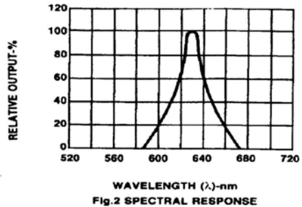
Fig. 2 SPECTRAL RESPONSE
