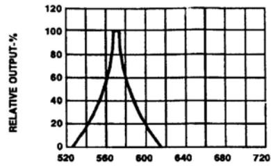
Fig.2 SPECTRAL RESPONSE
