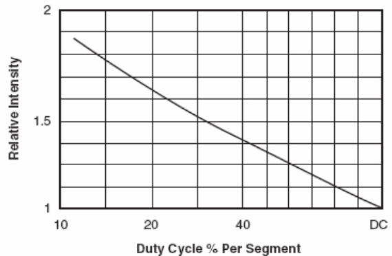
Fig. 5 Luminous Intensity vs. Duty Cycle
