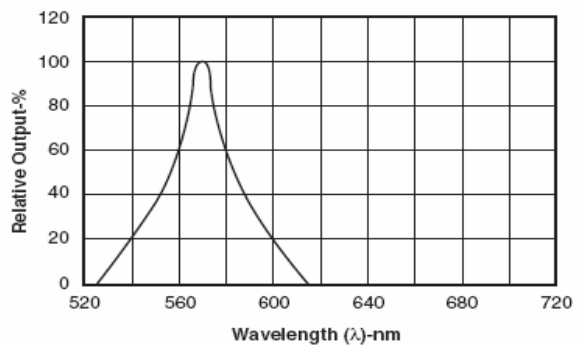
Fig. 2 Spectral Response
