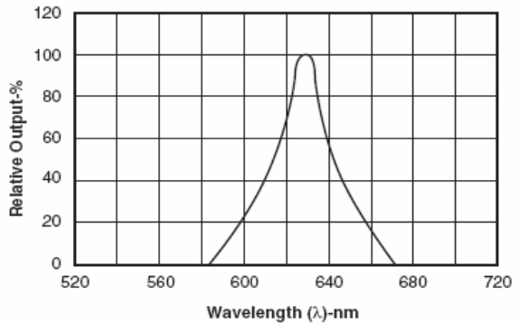
Fig. 2 Spectral Response
