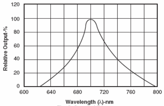
Fig. 2 Spectral Response
