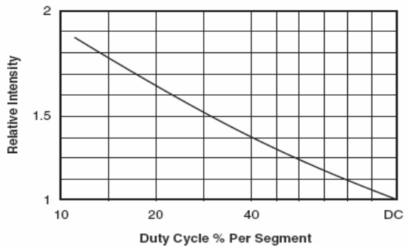
Fig. 5 Luminous Intensity vs. Duty Cycle
