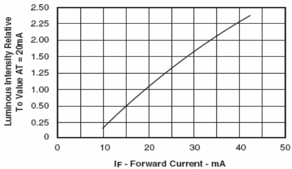
Fig. 3 Relative Luminous Intensity vs. Forward Current
