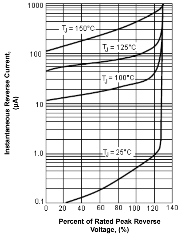
Typical Reverse Characteristics
