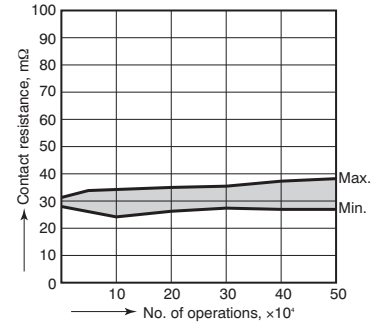
Change of contact resistance
