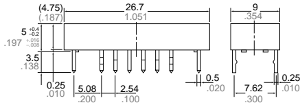
Self-clinching terminal
