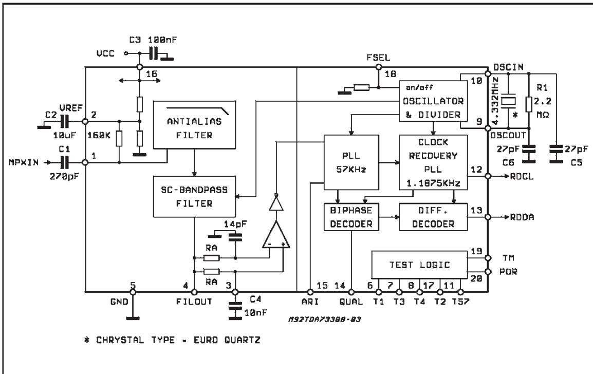
Figure 3: Test Circuit
