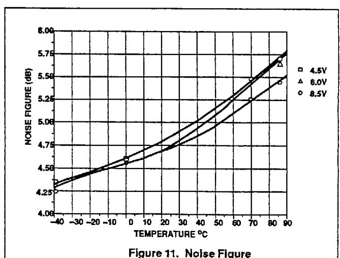
Figure 11. Noise Figure
