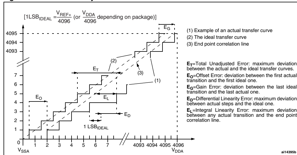
Figure 36. ADC accuracy characteristics
