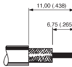
Part Number: 192945-4930
