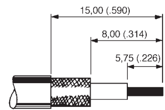
Part Number: 192945-4530
