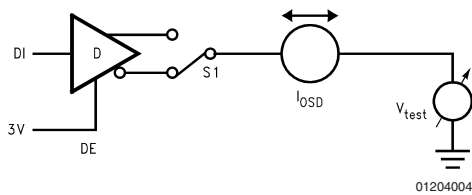
FIGURE 4. Driver I_{OSD}
