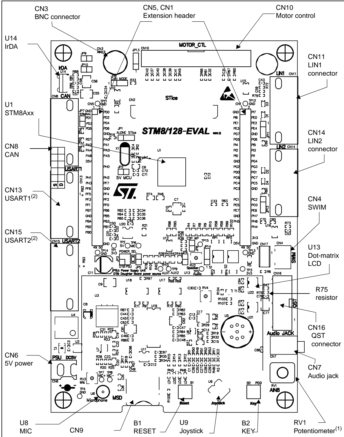
Figure 3. STM8A/128-EVAL evaluation board top layout
