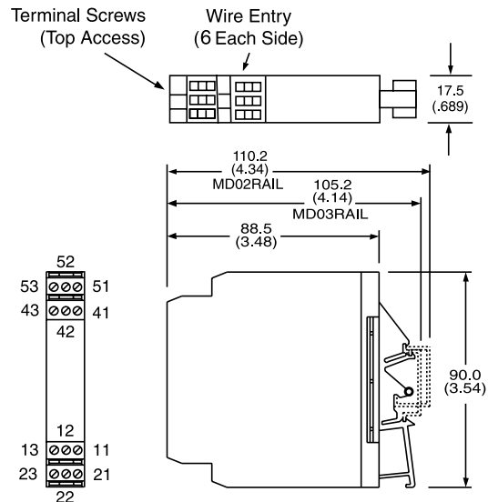
Dimensions are in mm (inches)
