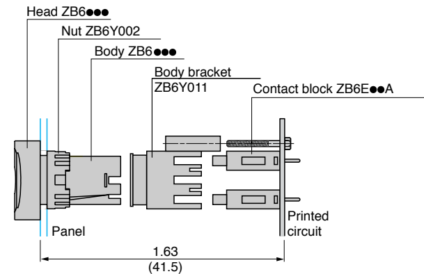
Direct mounting without socket adaptor ZB6Y010
