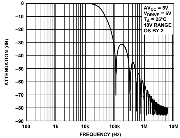
Figure 54. Digital Filter Response for OS × 2
