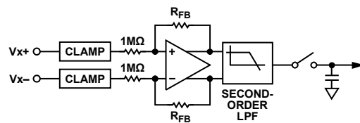
Figure 32. Analog Input Circuitry
