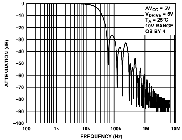
Figure 55. Digital Filter Response for OS × 4
