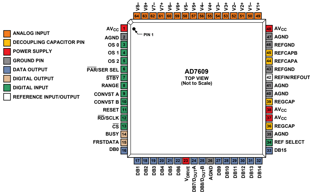
Figure 7. Pin Configuration
