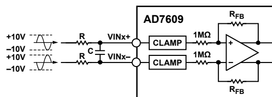
Figure 34. Input Resistance Matching on the Analog Input
