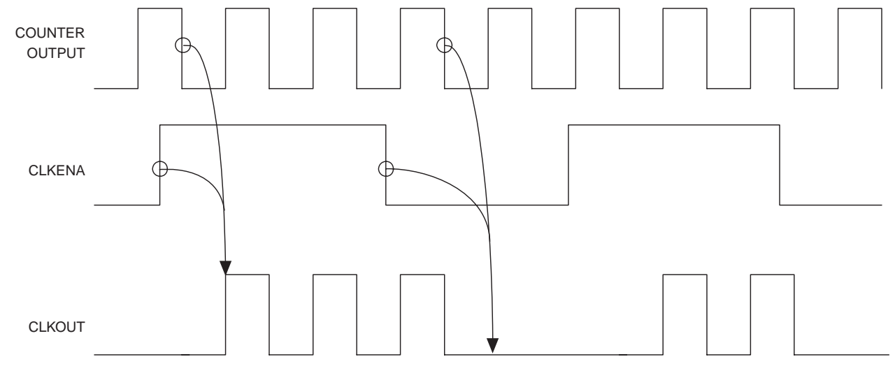
Figure 2–57. extclkena Signals
