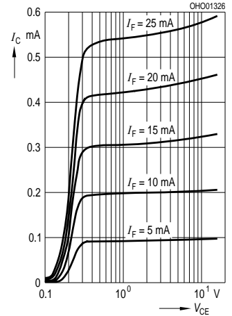
Output Characteristics (typ.) I_C = f(V_{CE}) , spacing d to reflector: d = 1\text{ mm}, 90\% reflection, T_A = 25^\circ\text{C}
