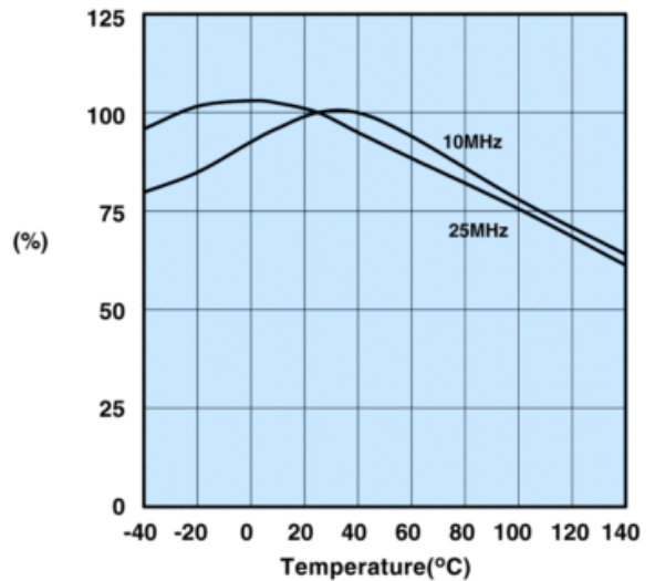
Measured on a 2673000301 using the HP4291A.
