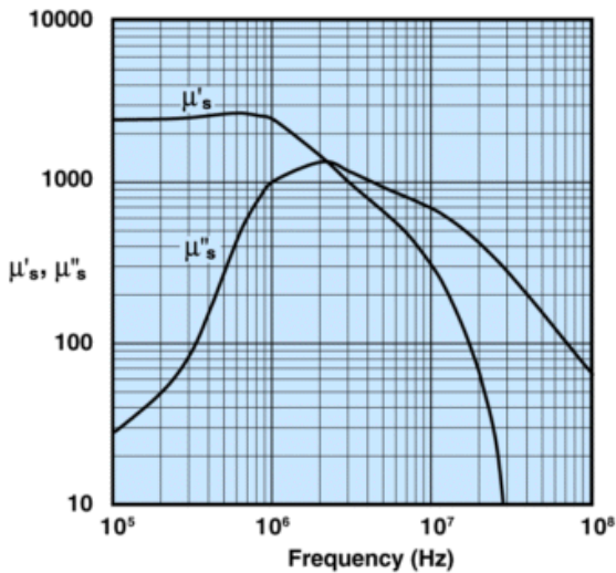
Measured on a 2673000301 bead using the HP 4284A and the HP 4291A.
