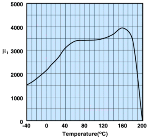
Measured on a 17/10/6mm toroid at 10kHz.
