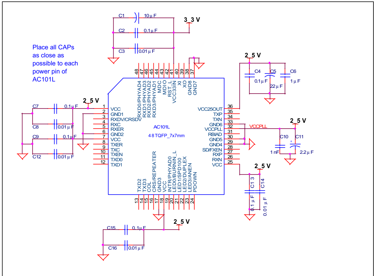
Figure 11: Power and ground filtering
