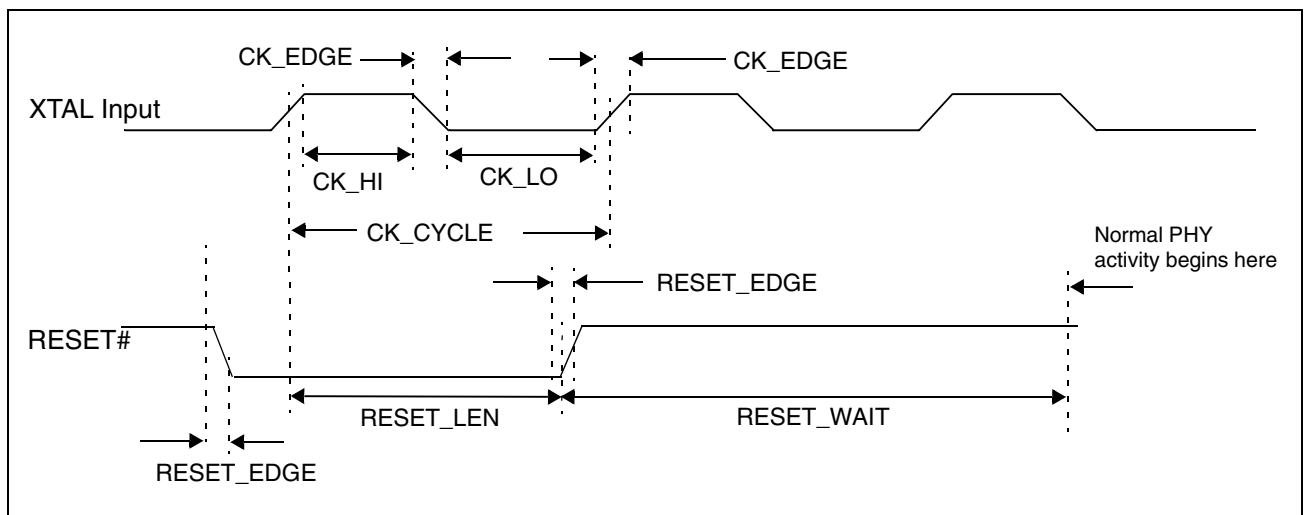
Figure 3: Reset Timing
