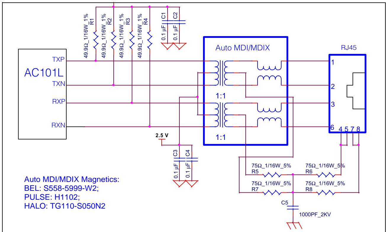
Figure 9: TX Application
