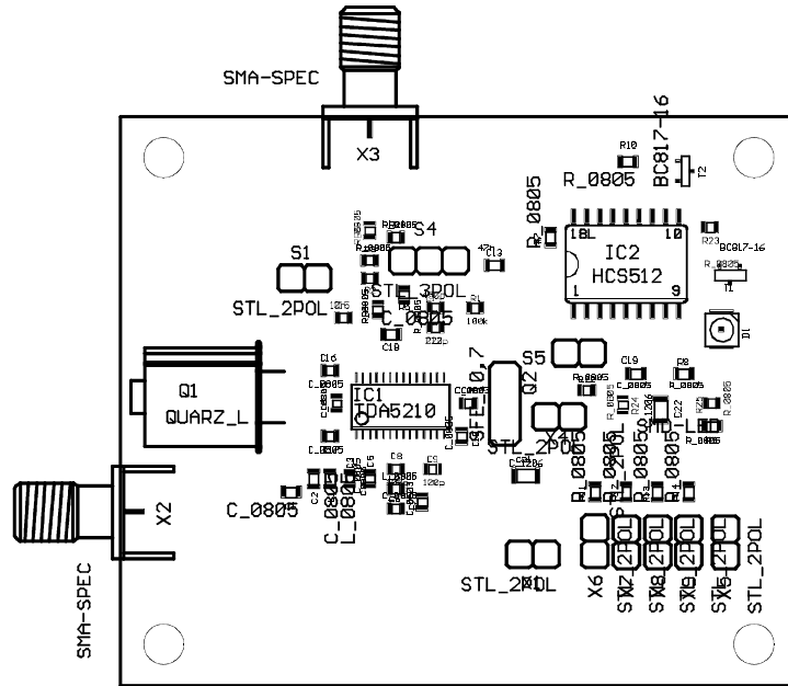
tda521x_testboard_20_plc.EMF
