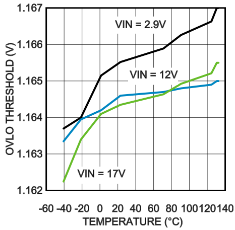
OVLO Threshold
