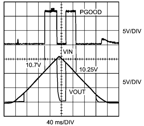
Startup (PGOOD)
