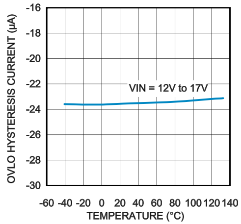
OVLO Hysteresis
