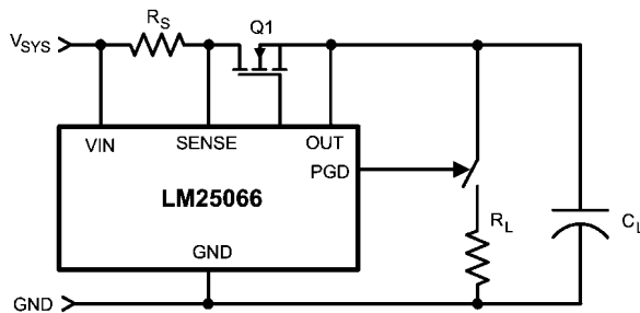
A. No Load Current During Turn-On
