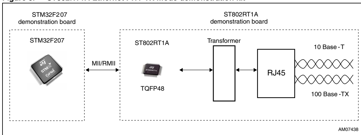
Figure 3. ST802RT1A Ethernet PHY TX mode demonstration kit
