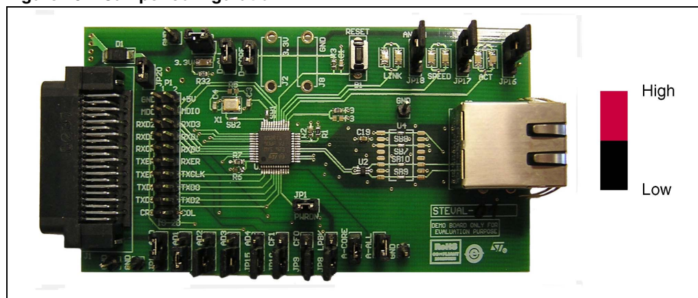
Figure 10. Jumper configuration
