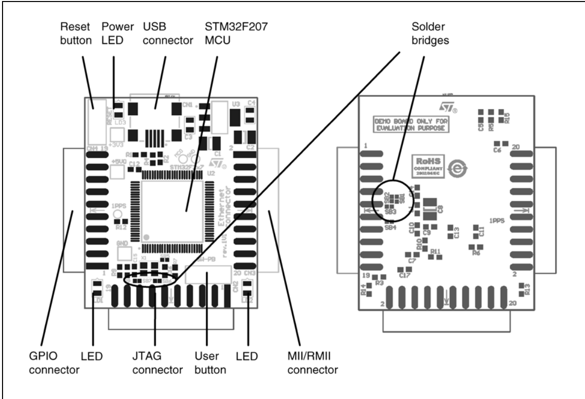
Figure 9. Board layout - STM32F207 controller demonstration board
